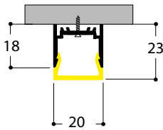
+ Section view without springs
