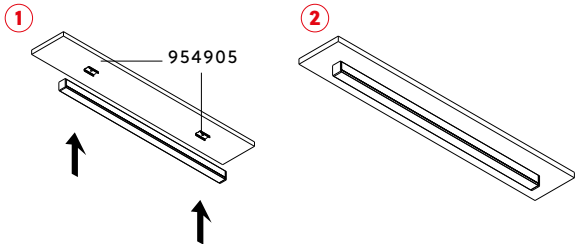
+ Fixation on surface
