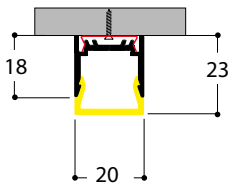
+ Section view with springs
