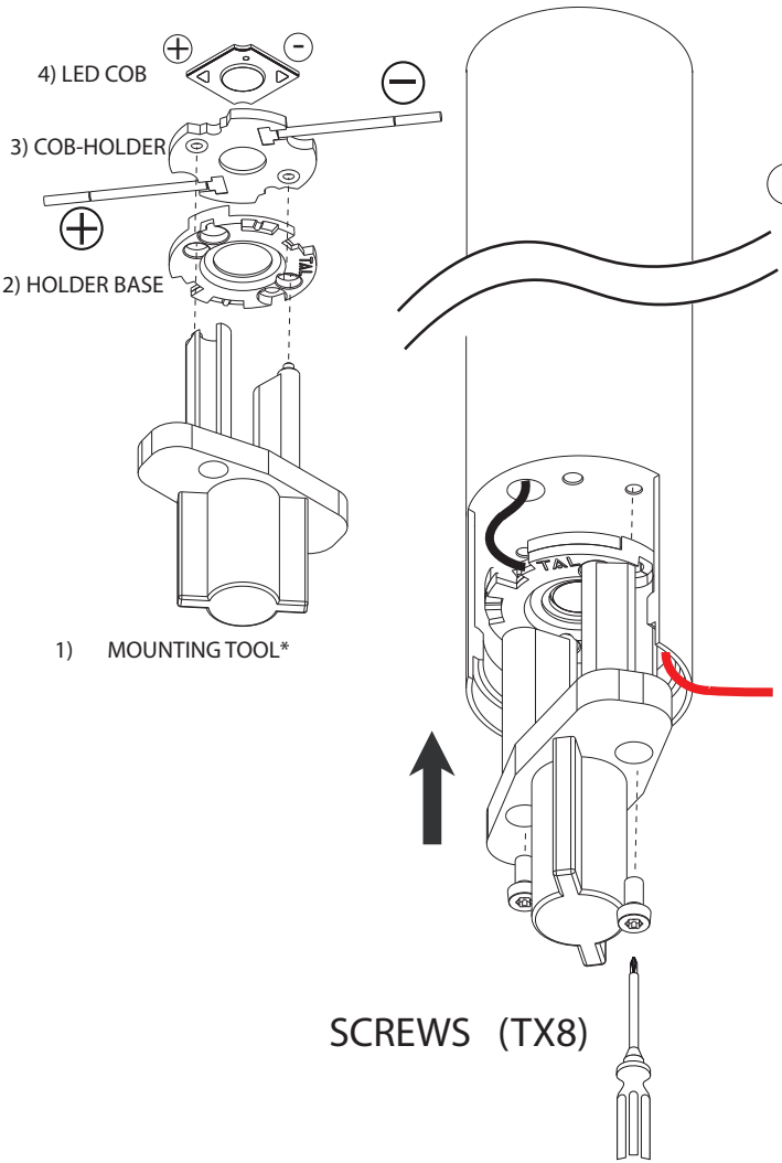
A Mounting led-parts into the lampfitting
