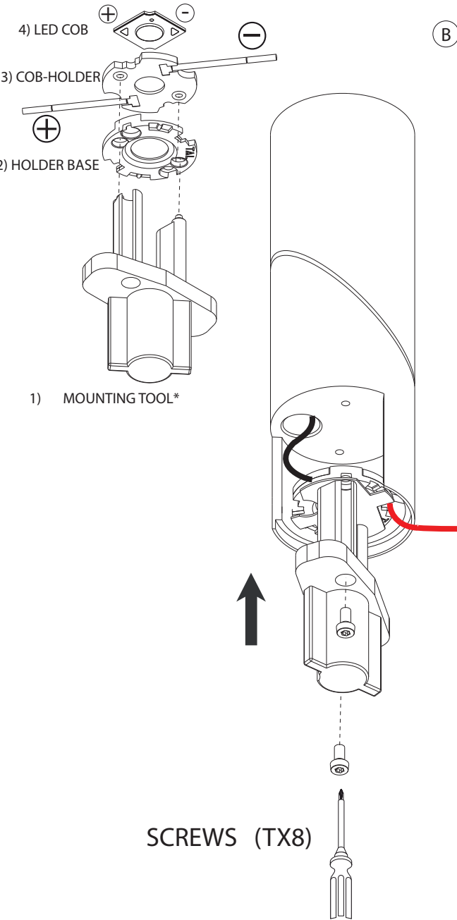
A Mounting led-parts into the lampfitting
